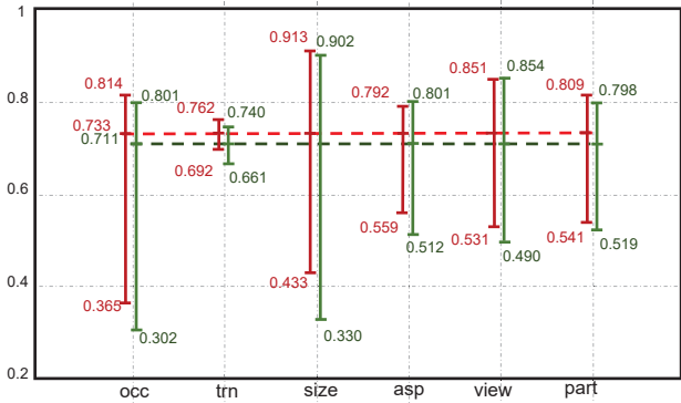
Figure 6. Summary of Sensitivity and Impact of Object Characteristics. We show the average (over 7 categories) Normalized AP ( AP_N [20]) of the highest performing and lowest performing subsets within each characteristic (occlusion, truncation, bounding box area, aspect ratio, viewpoint, part visibility). Overall AP_N is indicated by the dashed line. The difference between max and min indicates sensitivity. The difference between max and overall indicates the impact. Red: Scene . Green: baseline.
