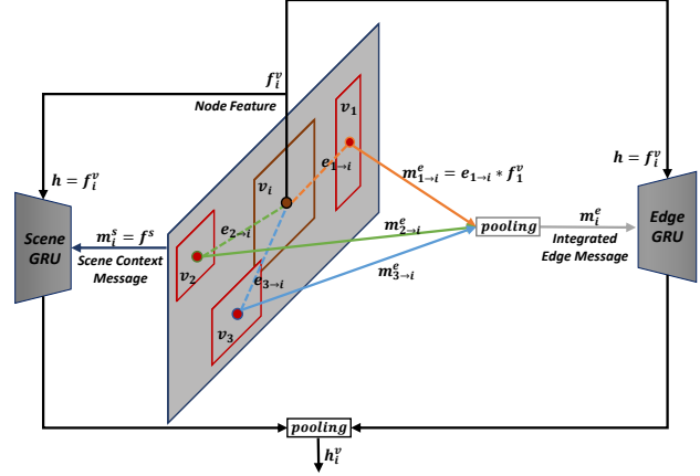
Figure 5. Structure Inference. For object v_i , the input of scene GRU is scene context message m_i^s , and the initial hidden state is the node v_i feature f_i^v . For message m_{1 \rightarrow i}^e from node v_1 to node v_i is controlled by edge e_{1 \rightarrow i} . These messages from all other objects are integrated as m_i^e to input the edge GRU. The initial hidden state of edge GRU is also f_i^v . Then these two sets of GRU output ensemble together as eventual updated node state.
